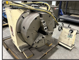
TSUDAKOMA RBA-500R 4TH AXIS ROTARY
