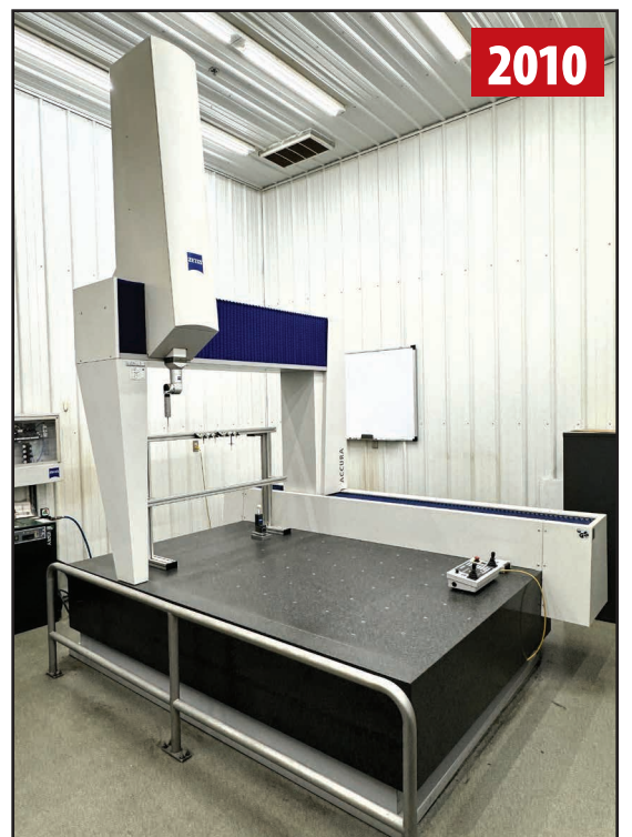
ZEISS ACCURA 12/18/10 COORDINATE MEASURING MACHINE
